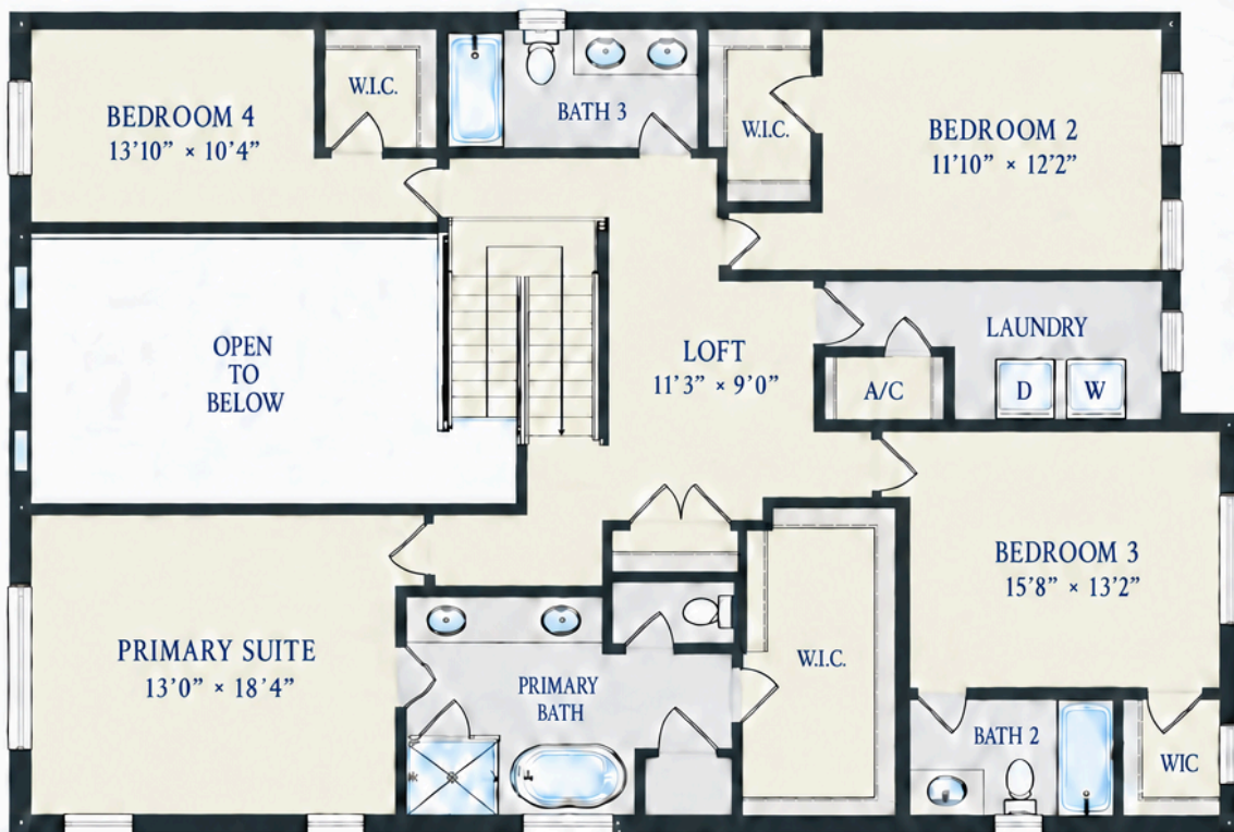
SECOND FLOOR
